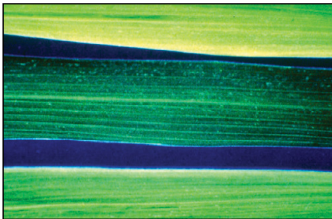
Varying degrees of Mo deficiency on rice
